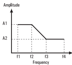
Bellcore GR-499 jitter amplitude versus modulation frequency:
