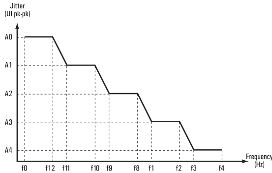
ITU-T Q.171 PDH jitter amplitude versus modulation frequency:
