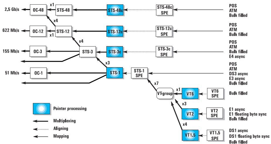
Figure 1: Bellcore GR-253 mapping structure (SONET payload mapping)
