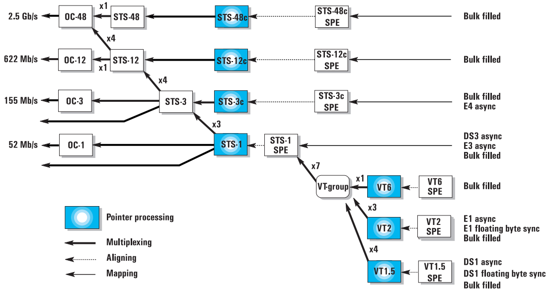
Figure 1: Bellcore GR-253 mapping structure (SONET payload mapping)
